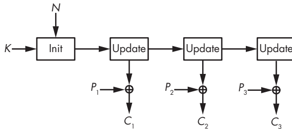
Figure 5-2: A stateful stream cipher
