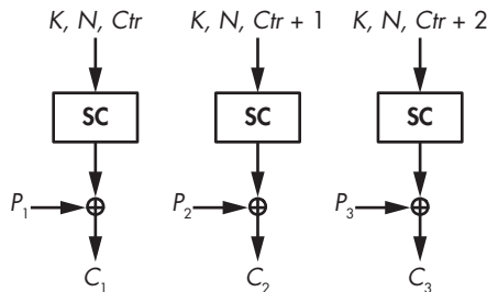
Figure 5-3: A counter-based stream cipher
