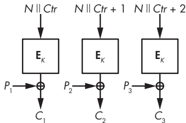
Figure 4-10: CTR mode
