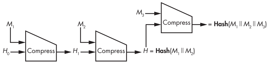
Figure 6-9: The length-extension attack
