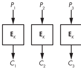
Figure 4-6: ECB mode
