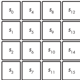
Figure 4-3: The internal state of AES as a 4x4 array of 16 bytes
