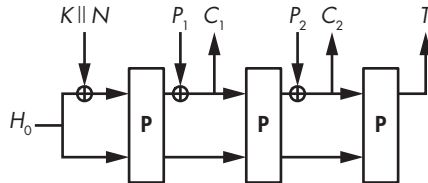
Figure 8-4: A permutation-based authenticated cipher
