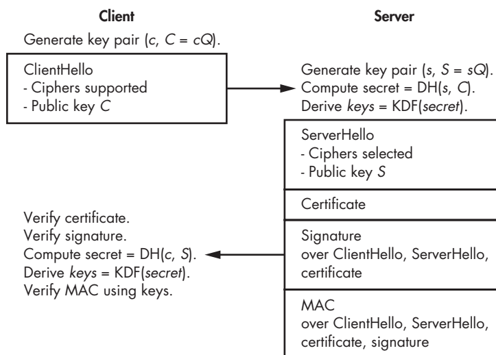
Figure 13-1: The TLS 1.3 handshake process
