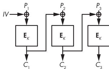
Figure 4-8: CBC mode
